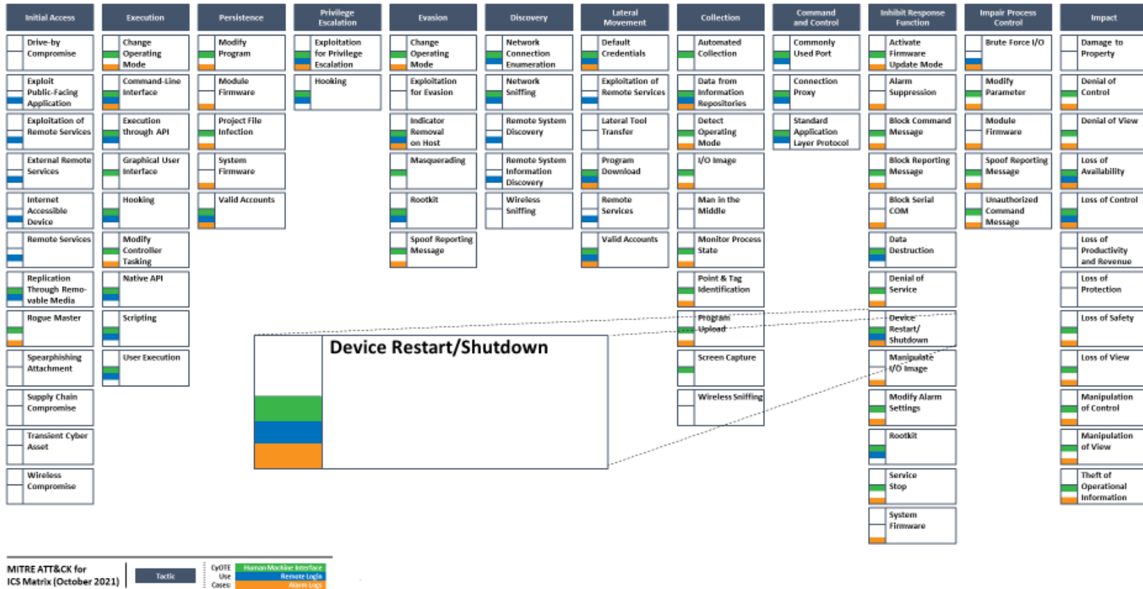
Figure 1: ICS ATT&CK Framework 9 – Device Restart/Shutdown Technique
